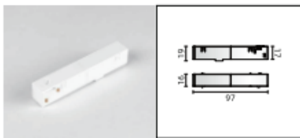
Live-end connector(Right)
