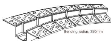
Alu profile (Pre-embedded) N016016-SMS-R-S-1M-A01
