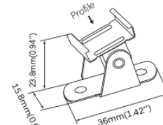
Adjustable bracket (Installation requires matching profile) CP07-90
