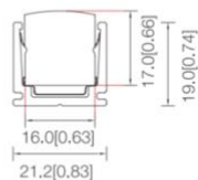
Aluminum channel (with metal spring)
