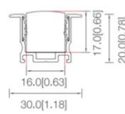
Aluminum channel with silicone (with wings)
