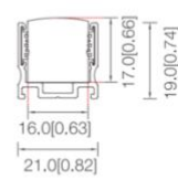
Aluminum channel with silicone (no-wings)
