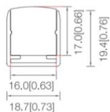
Aluminum channel (Aluminum clip)
